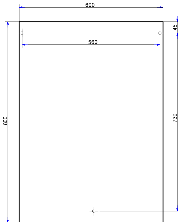
СВТ64.830.000-02 (..-03) [50, 95А]
